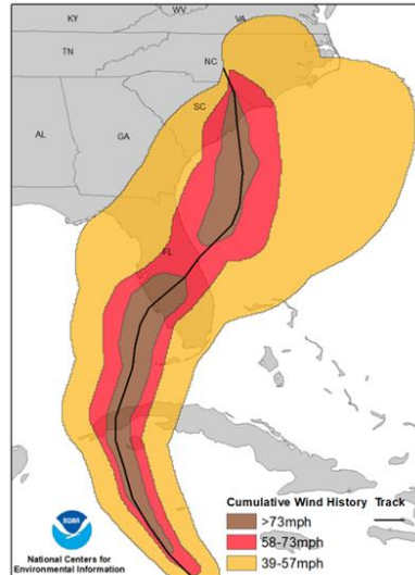
Figure 2. Hurricane Ian Track and Wind History
