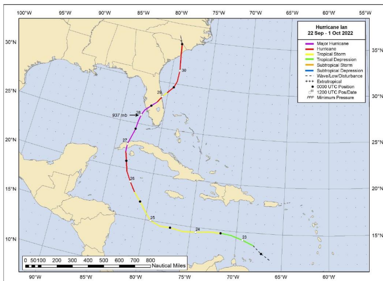
Figure 1. Best Track Position for Hurricane Ian, September 23-30, 2022
